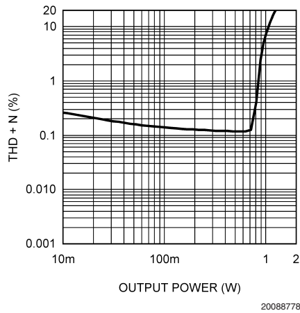
THD+N vs Output Power 3V, 8Ω, SE at 1kHz
