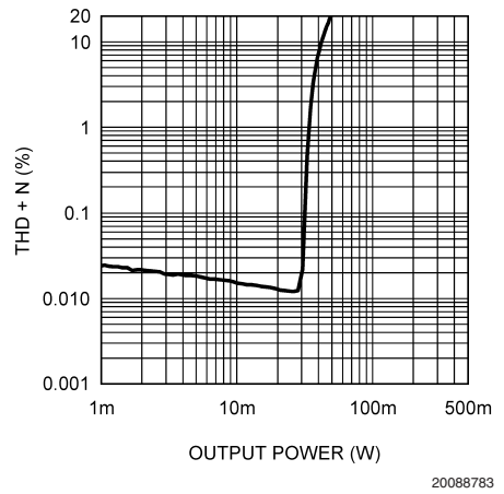
THD+N vs Output Power 3V, 32Ω, SE at 1kHz
