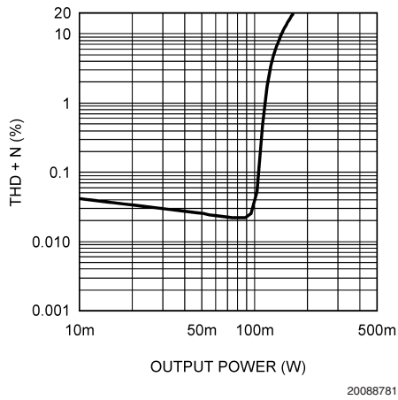
THD+N vs Output Power 3V, 8Ω, SE at 1kHz
