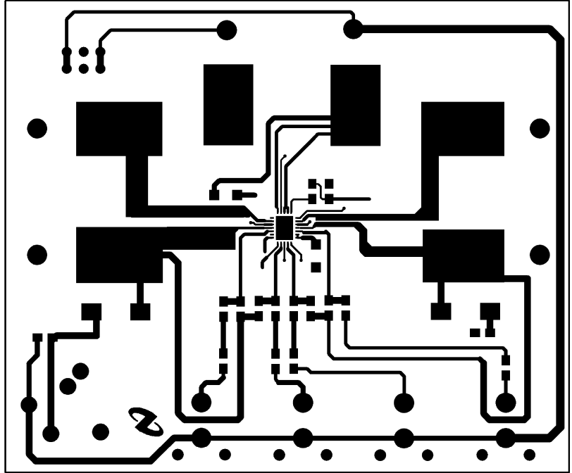
FIGURE 5. Top Layer
