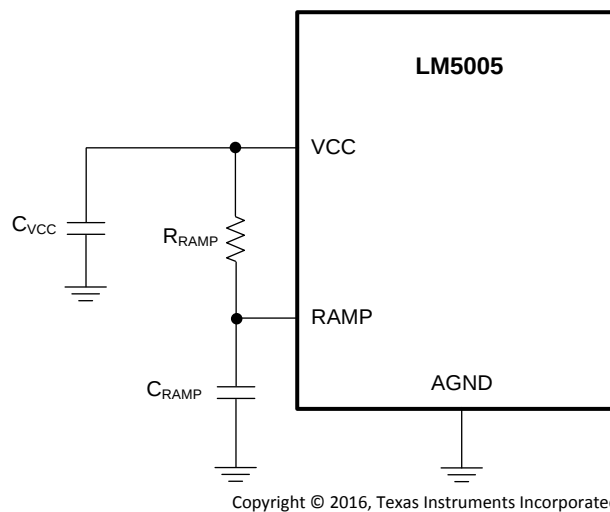
Figure 13. Connection of External Ramp Resistor to VCC when V_{OUT} > 7.5 V
