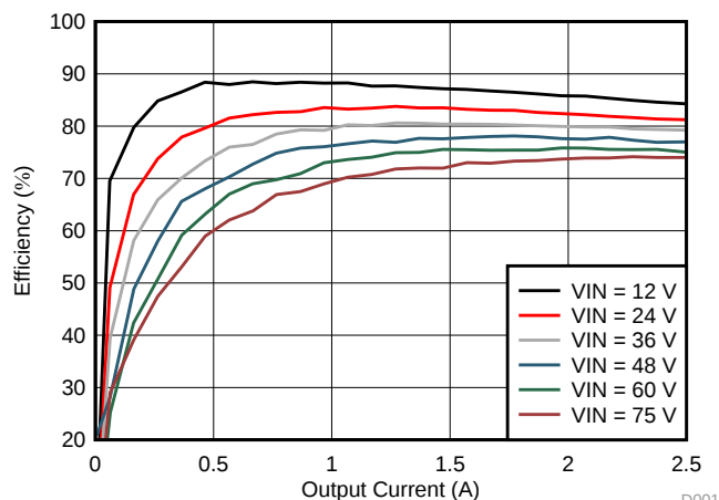
Typical Efficiency, V_{\text{OUT}} = 5 \text{ V}
