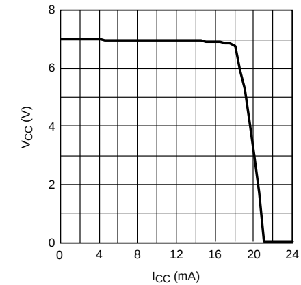
Figure 4. V_{CC} vs I_{CC}
