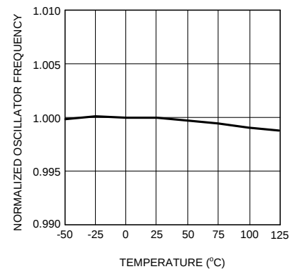
Figure 2. Oscillator Frequency vs Temperature
