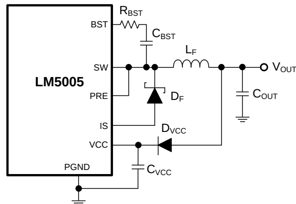
Figure 14. VCC Bias From the Output Voltage for 8 V < V OUT < 14 V
