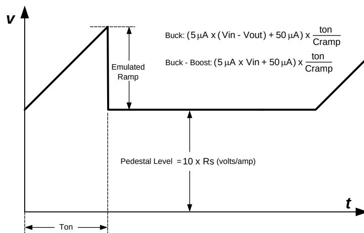
Figure 13. Composition of Emulated Current Signal
