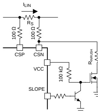
Figure 36. Inrush Current Limit Programming #2
