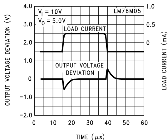
Figure 10. Load Transient Response
