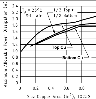
Figure 14. Maximum Allowable Power Dissipation vs 2-oz Copper Area for PFM
