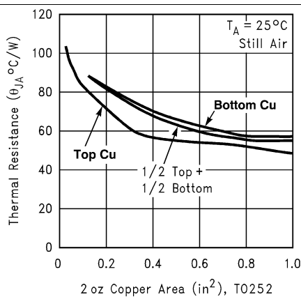
Figure 12. R_{\theta JA} vs 2-oz Copper Area for PFM
