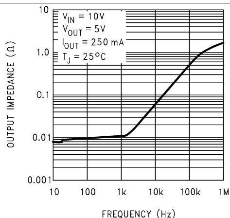
Figure 8. Output Impedance
