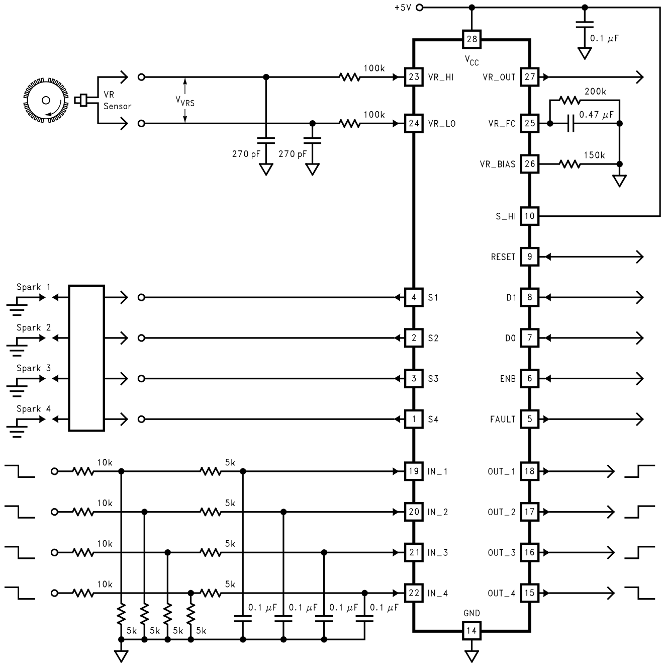
Figure 24. Typical Application
