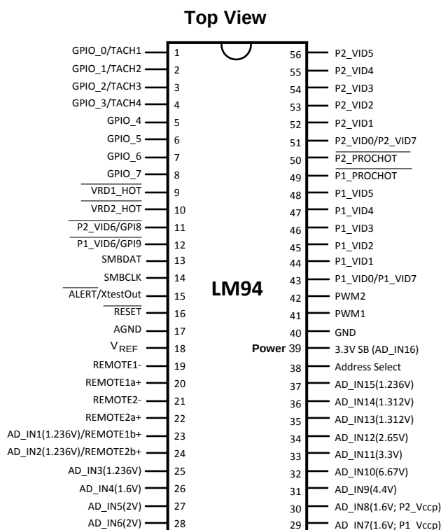
Figure 2. 56 Pin TSSOP Package See Package Number DGG0056A
