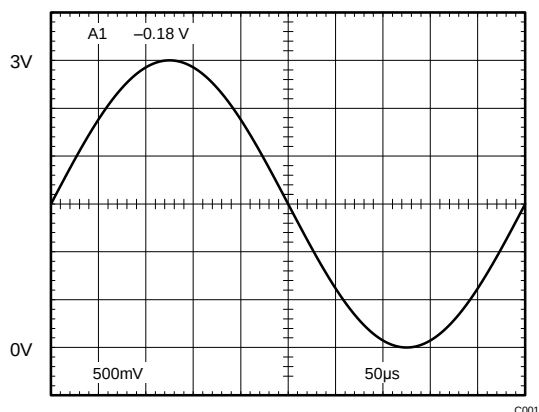
Rail-to-Rail Input
