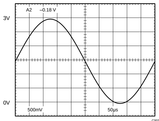
Rail-to-Rail Output
