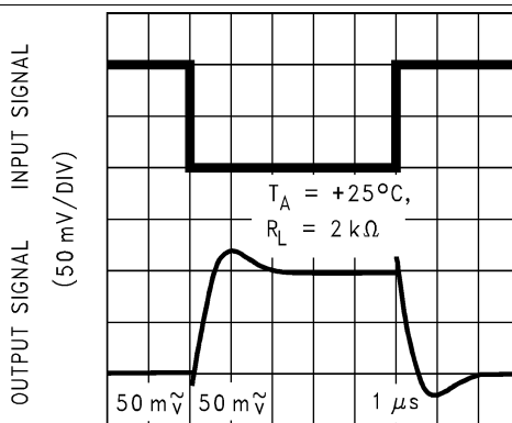
TIME (1 μs/DIV) Figure 44. Inverting Small Signal Pulse Response
