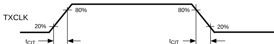
Figure 3. Transmit Clock Transition Times
