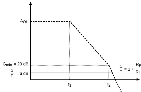
Figure 53. 1/F for R_F = R_1 and Open Loop Gain Plot
