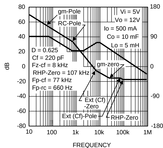
Figure 18. LMR62421 With External Compensation
