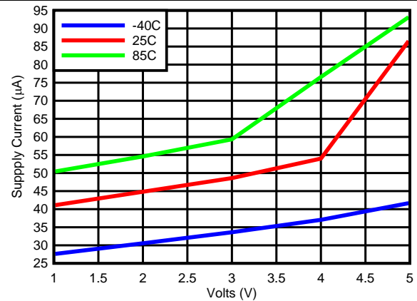
Figure 2. Supply Current vs Supply Voltage Output Low (LMV33x)
