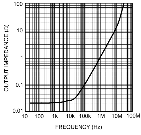
Figure 34. Closed-Loop Output Impedance vs Frequency
