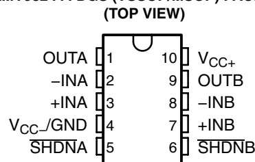
LMV982 . . . DGS (VSSOP/MSOP) PACKAGE
