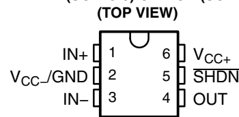
LMV981 . . . RUG (QFN) PACKAGE
