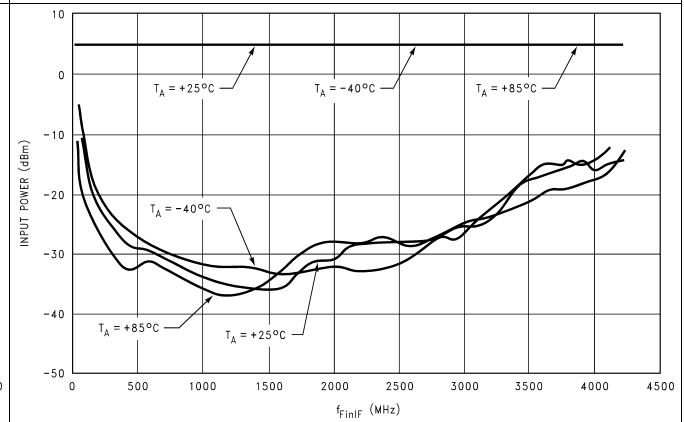
Figure 12. LMX2434 FinIF Input Power vs Frequency
