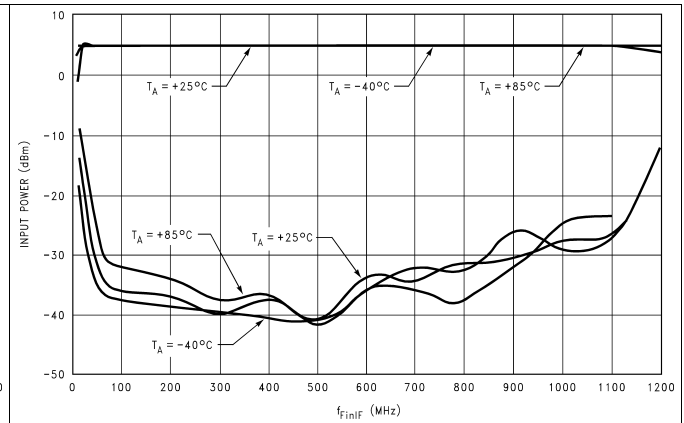
Figure 8. LMX2430 FinIF Input Power vs Frequency
