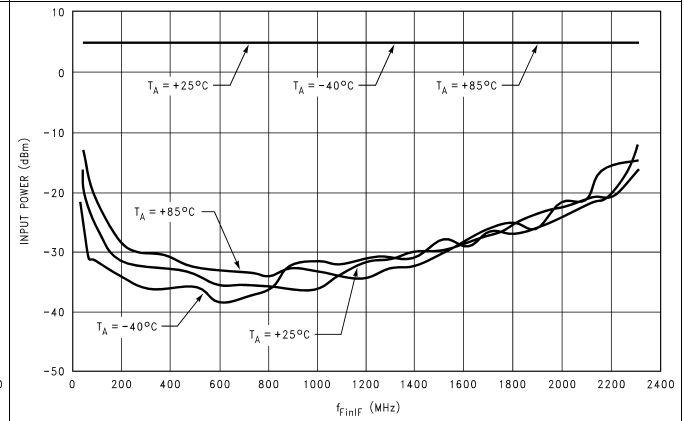
Figure 10. LMX2433 FinIF Input Power vs Frequency
