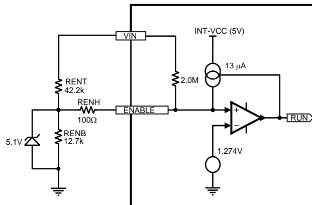
Figure 48. Enable Input Detail
