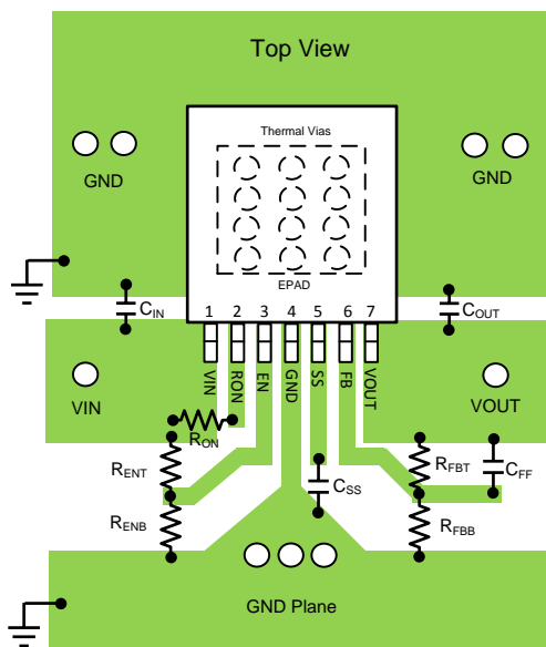
Figure 40. PCB Layout Guide
