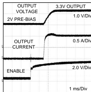
Figure 31. Prebiased Start-Up
