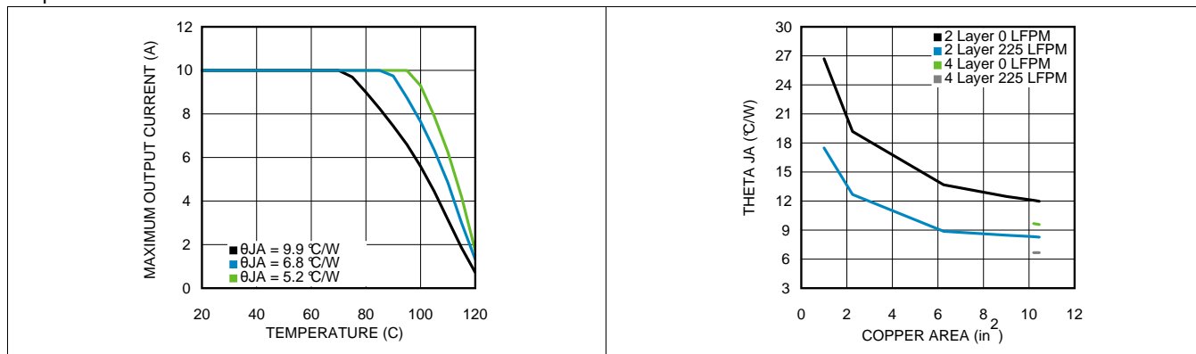
Figure 31. Thermal Derating
