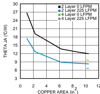
Figure 32. \theta_{JA} vs Copper Heat Sinking Area
