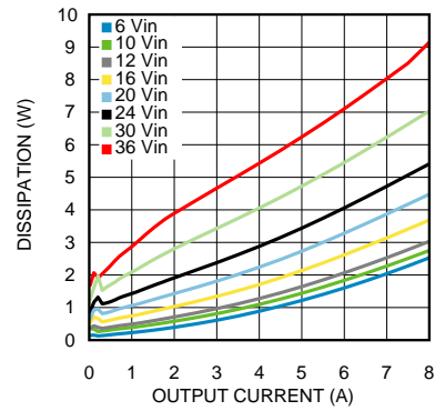
Figure 14. Dissipation 1-V Output at 25°C
