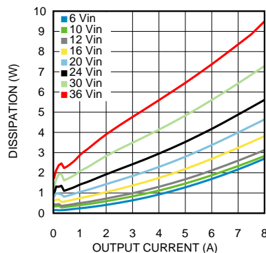
Figure 8. Dissipation 1.8-V Output at 25°C
