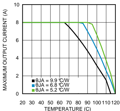
Figure 31. Thermal Derating
