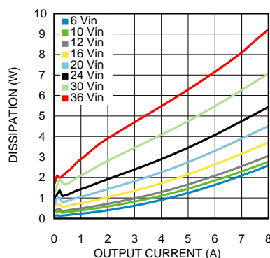
Figure 10. Dissipation 1.5-V Output at 25°C
