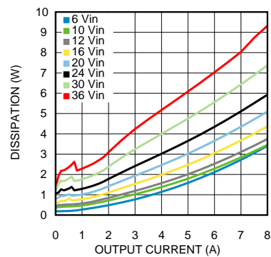
Figure 16. Dissipation 5-V Output at 85°C
