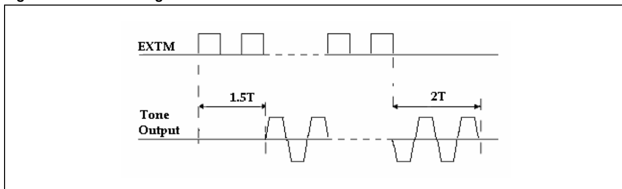
Figure 2. EXTM timings
