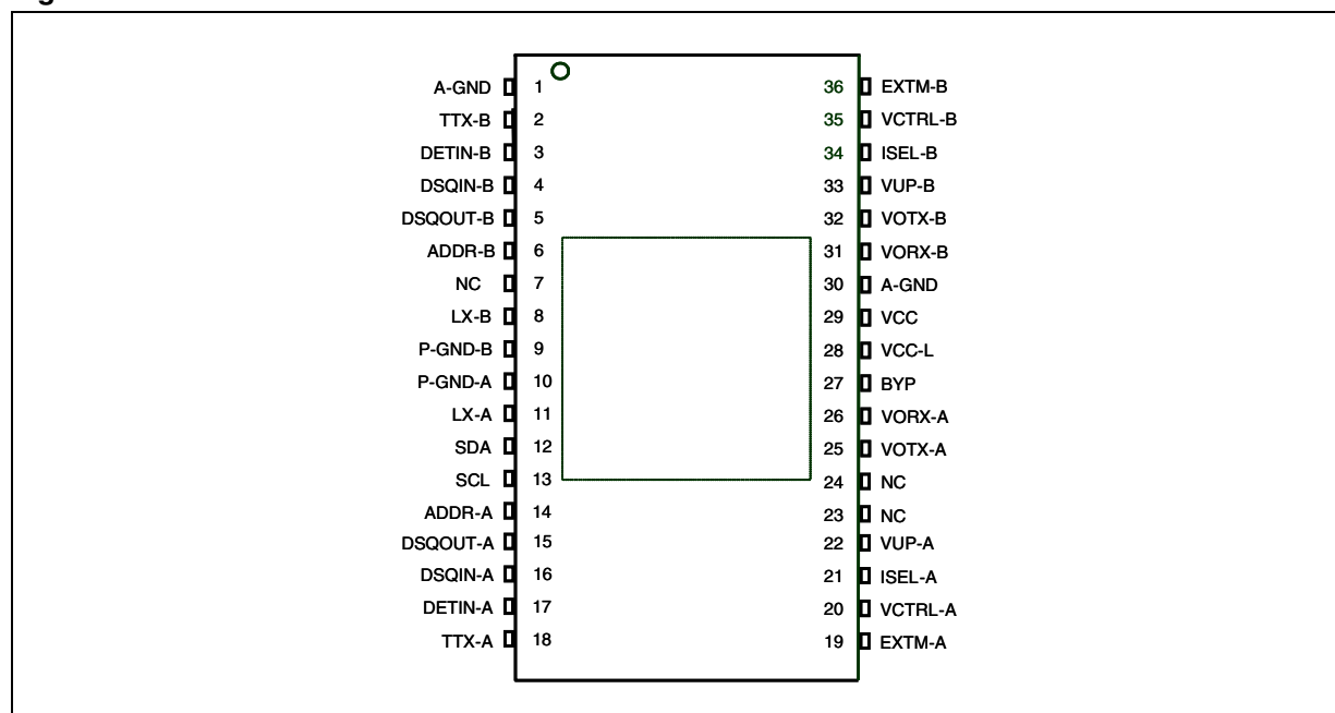
Figure 3. Pin connections
