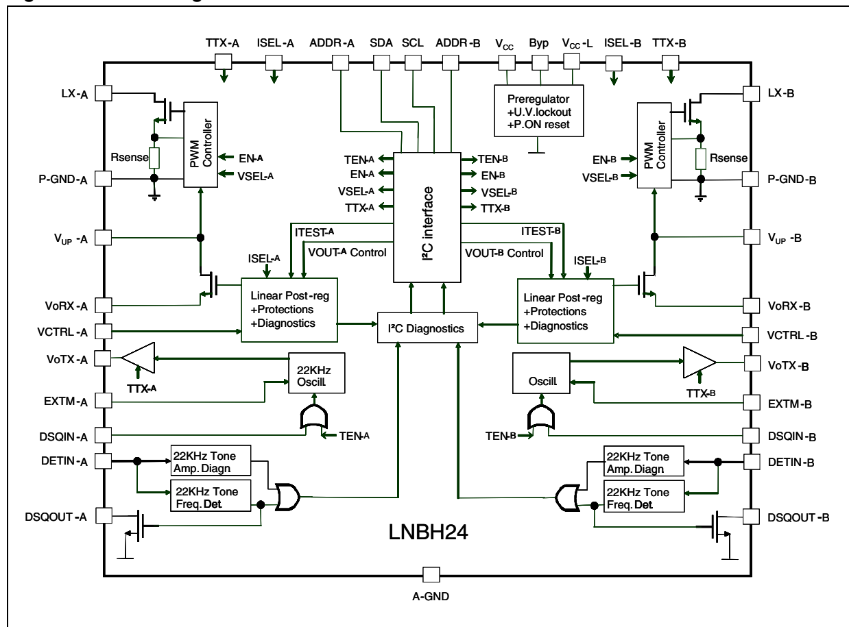
Figure 1. Block diagram
