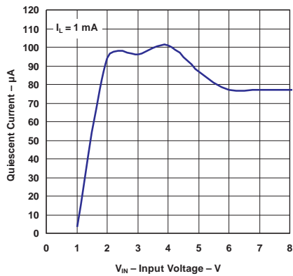
Figure 7. Quiescent Current vs Input Voltage
