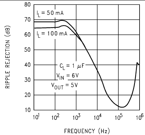
Figure 22. Ripple Rejection
