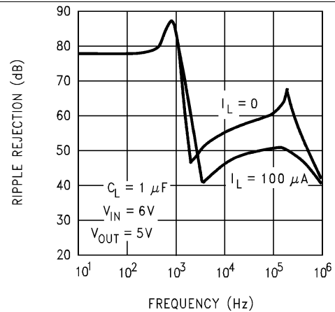
Figure 20. Ripple Rejection
