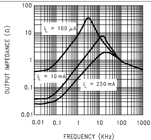
Figure 12. Output Impedance
