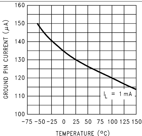
Figure 2. Quiescent Current
