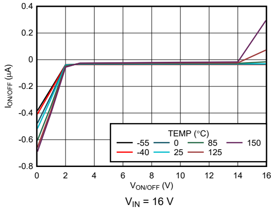
Figure 5-39. ON/\overline{OFF} Pin Current vs V_{ON/OFF} (New Chip)
