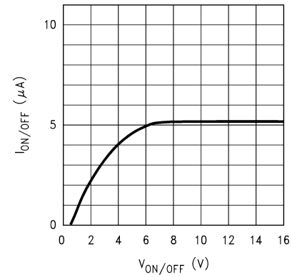
Figure 5-38. ON/\overline{OFF} Pin Current vs V_{ON/OFF} (Legacy Chip)
