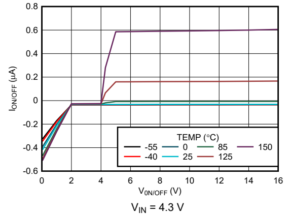
Figure 5-40. ON/\overline{OFF} Pin Current vs V_{ON/OFF} (New Chip)
