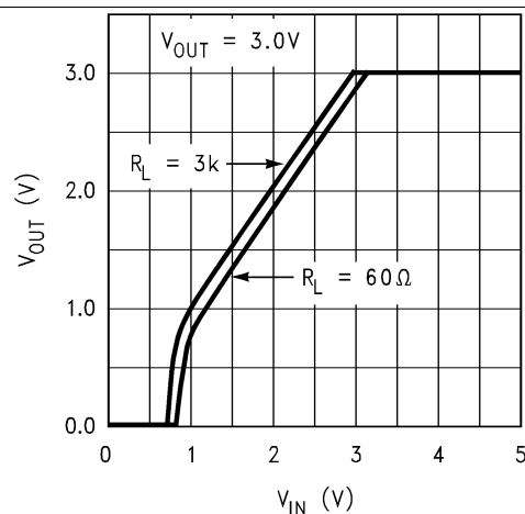
Figure 6. Dropout Characteristics
