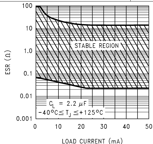
Figure 32. 2.2- \mu F ESR Range
