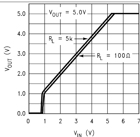
Figure 4. Dropout Characteristics
