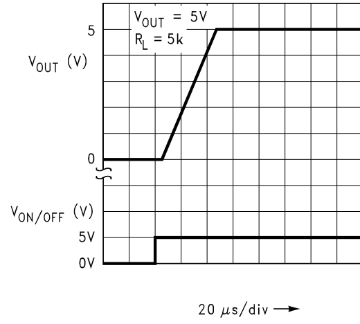
Figure 28. Turnon Waveform
