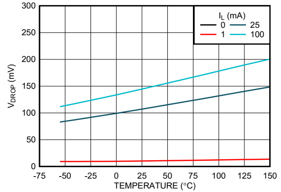
Figure 5-8. Dropout Voltage ( V_{DO} ) vs Temperature (New Chip)
