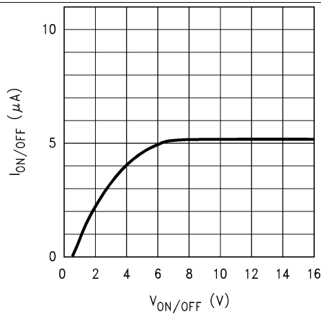
Figure 31. ON/OFF Pin Current vs V_{\text{ON}/\overline{\text{OFF}}}
