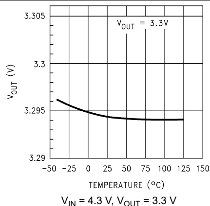
Figure 5-2. Output Voltage versus Temperature (Legacy Chip)
