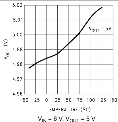
Figure 5-1. Output Voltage versus Temperature (Legacy Chip)
