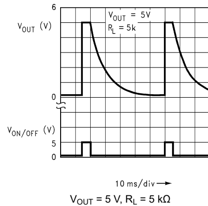
Figure 7-18. Turn-off Waveform (Legacy Chip)
