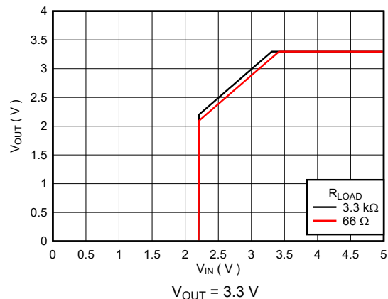
Figure 5-8. Output Voltage versus V_{IN} (New Chip)
