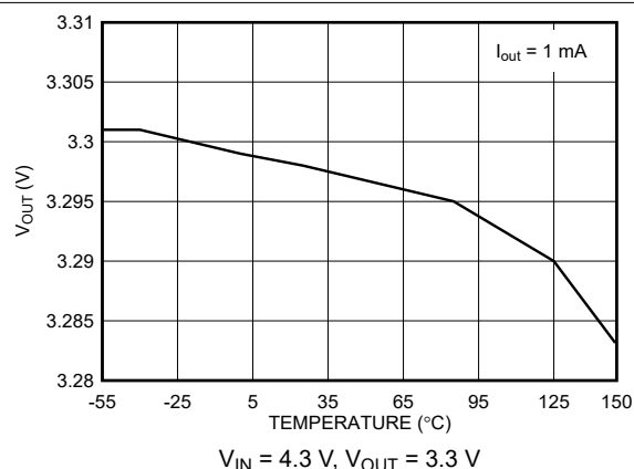
Figure 5-4. Output Voltage versus Temperature (New Chip)
