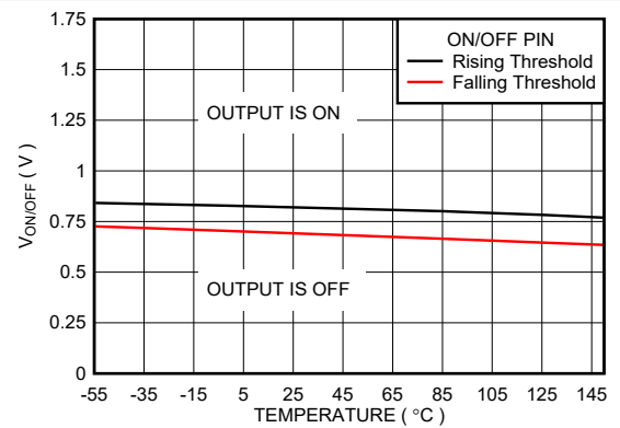
Figure 5-58. ON/ OFF Threshold versus Temperature (New Chip)
