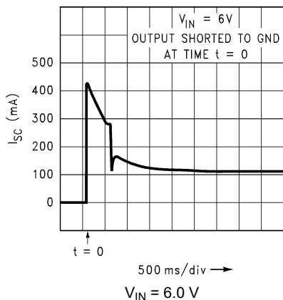
Figure 5-31. Short Circuit Current versus Time (Legacy Chip)
