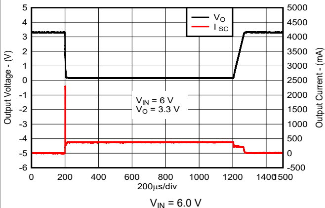
Figure 5-32. Short Circuit Current versus Time (New Chip)
