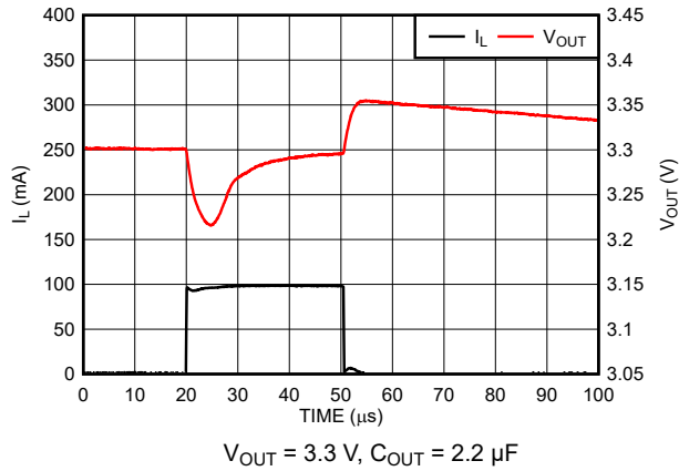
Figure 7-15. Load Transient Response (New Chip)
