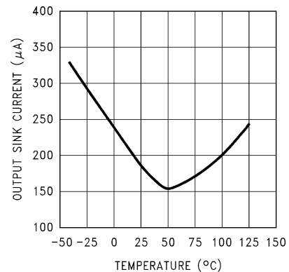
Figure 5-48. Output Reverse Leakage versus Temperature (Legacy Chip)
