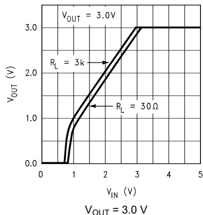
Figure 5-7. Output Voltage versus V_{IN} (Legacy Chip)
