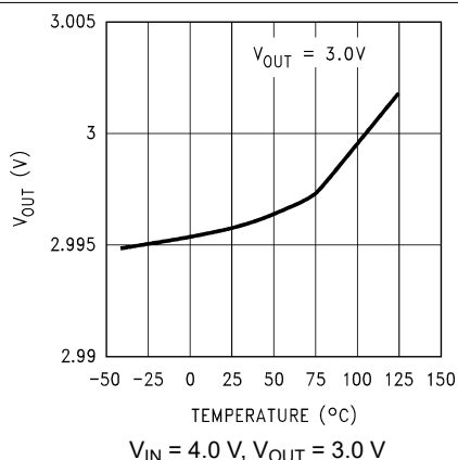
Figure 5-3. Output Voltage versus Temperature (Legacy Chip)
