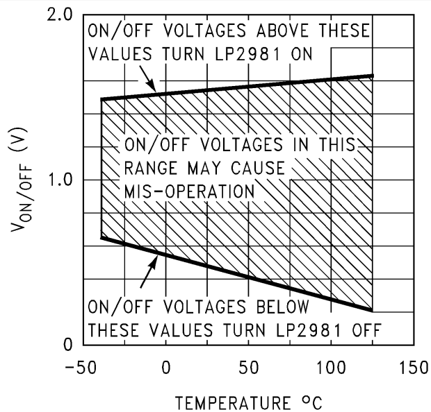
Figure 5-57. ON/ OFF Threshold versus Temperature (Legacy Chip)
