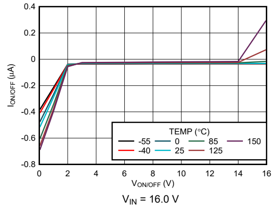
Figure 5-56. ON/ OFF Pin Current versus V_{ON/OFF} (New Chip)
