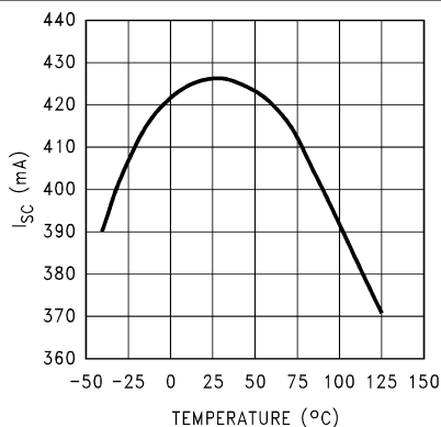
Figure 5-35. Instantaneous Short Circuit Current versus Temperature (Legacy Chip)
