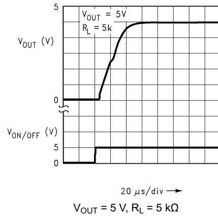
Figure 7-16. Turn-on Waveform (Legacy Chip)
