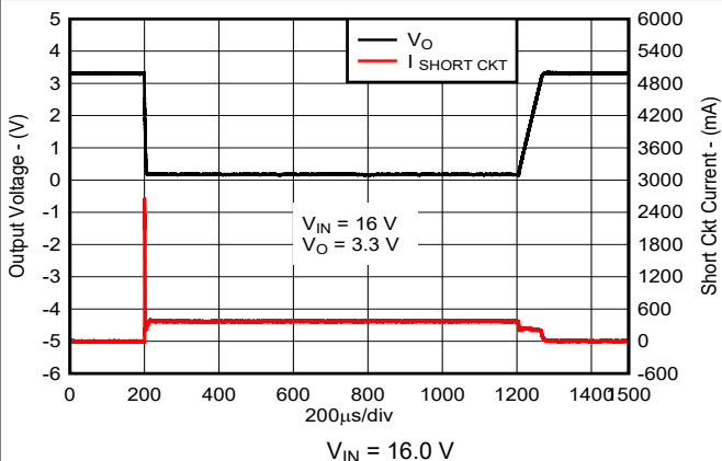
Figure 5-34. Short Circuit Current versus Time (New Chip)
