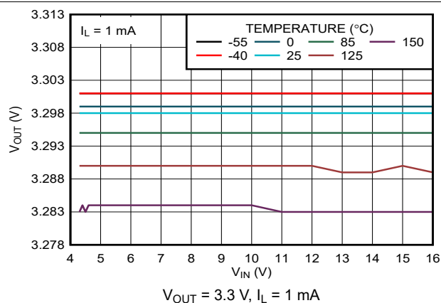
Figure 5-9. Output Voltage versus V_{IN} and Temperature (New Chip)
