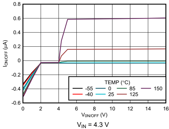
Figure 5-55. ON/ OFF Pin Current versus V_{ON/OFF} (New Chip)
