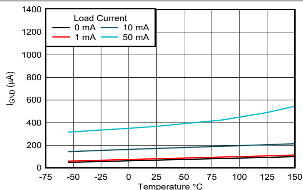
Figure 5-16. Ground Pin Current ( I_{GND} ) versus Temperature (New Chip)
