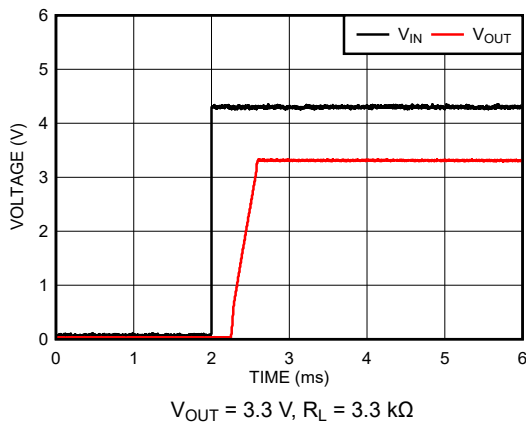
Figure 7-17. Turn-on Waveform (New Chip)
