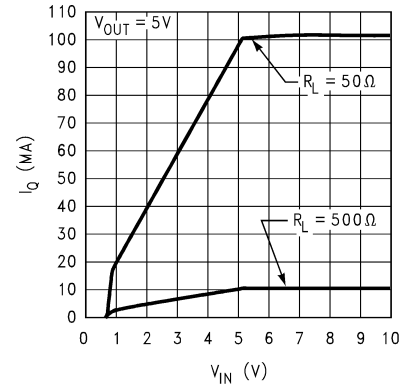
Figure 5-20. Input Current versus Input Voltage ( V_{IN} ) (Legacy Chip)
