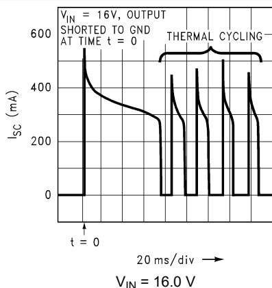
Figure 5-33. Short Circuit Current versus Time (Legacy Chip)
