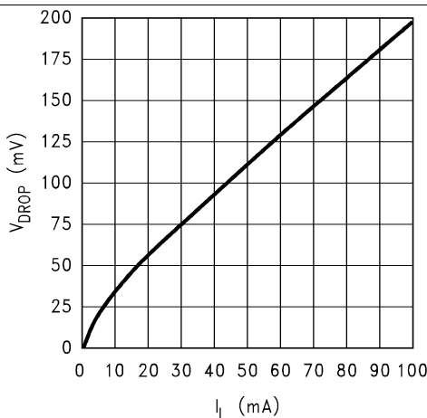
Figure 8. Dropout Voltage vs Load Current
