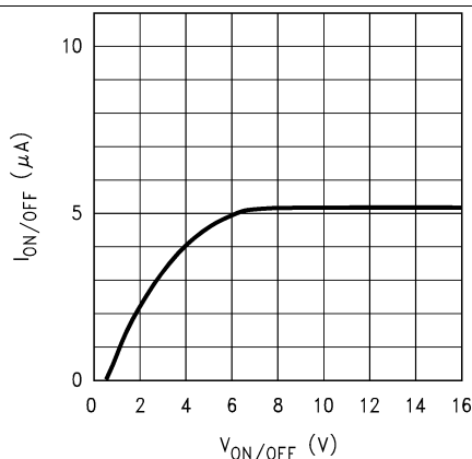
Figure 25. ON/ \overline{\text{OFF}} Pin Current vs V_{ON/OFF}
