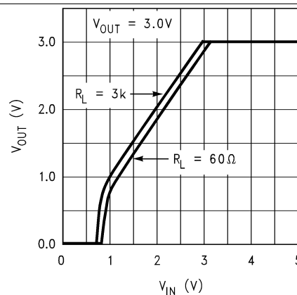
Figure 4. Dropout Characteristics
