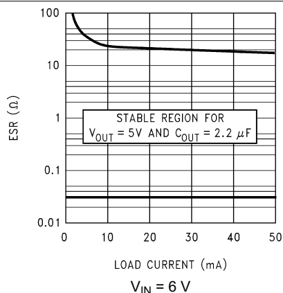
Figure 7-3. 5-V, 2.2- \mu F ESR Curves (Legacy chip)
