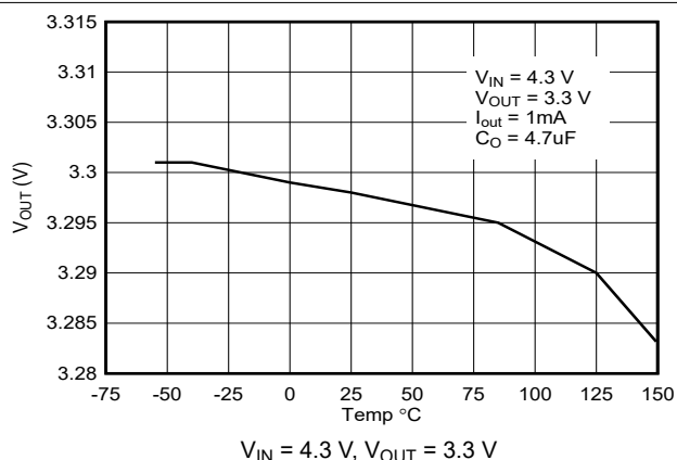
Figure 5-4. Output Voltage versus Temperature (New Chip)
