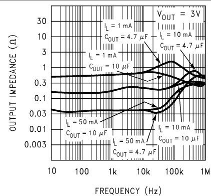
Figure 5-36. Output Impedance versus Frequency (Legacy chip)
