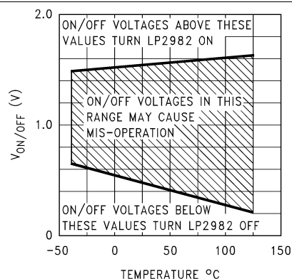
Figure 5-40. ON/ OFF Threshold versus Temperature (Legacy chip)
