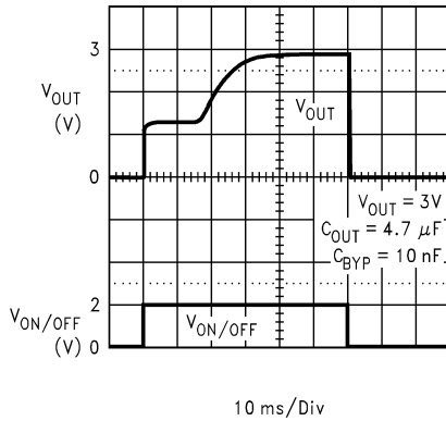
Figure 5-55. Turnon Waveform (Legacy chip)
