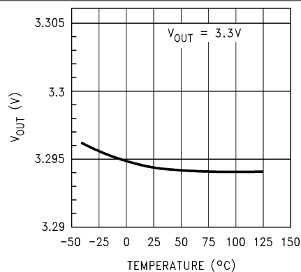
Figure 5-2. Output Voltage versus Temperature (Legacy Chip)
