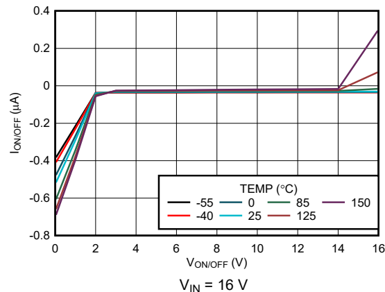
Figure 5-38. ON/ OFF Pin Current versus V_{ON/OFF} (New Chip)
