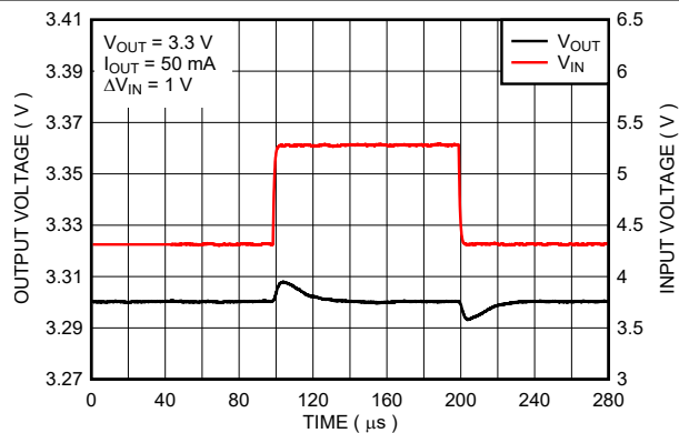
Figure 7-7. Line Transient Response (New Chip)
