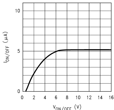
Figure 5-37. ON/ OFF Pin Current versus V_{ON/OFF} (Legacy chip)
