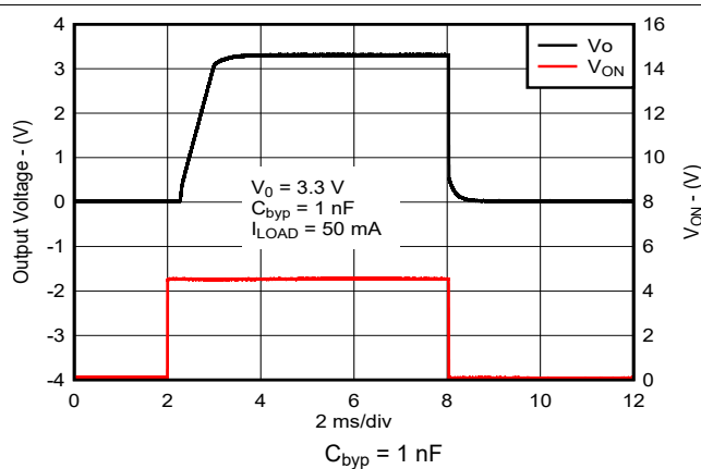
Figure 7-18. Turnon Waveform (New chip)
