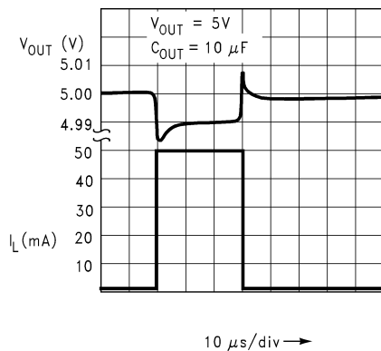
Figure 7-11. Load Transient Response (Legacy chip)
