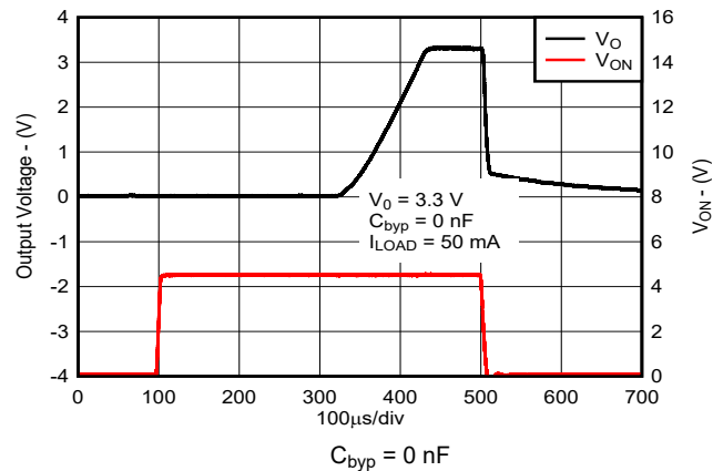
Figure 7-16. Turnon Waveform (New chip)
