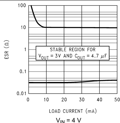
Figure 7-4. 3-V, 4.7- \mu F ESR Curves (Legacy chip)
