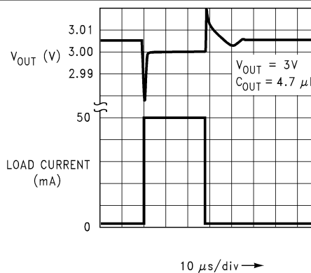
Figure 7-8. Load Transient Response (Legacy chip)
