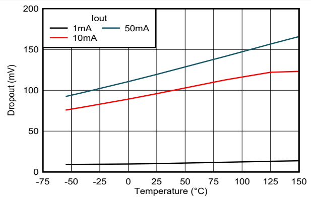
Figure 5-10. Dropout Voltage versus Temperature (New Chip)
