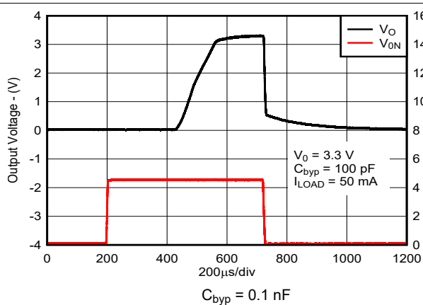
Figure 7-17. Turnon Waveform (New chip)
