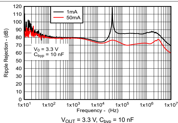
Figure 5-52. Ripple Rejection versus I_{OUT} (New Chip)
