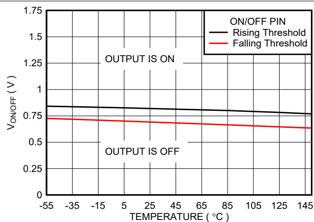
Figure 5-41. ON/ OFF Threshold versus Temperature (New chip)
