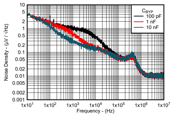
Figure 5-48. Output Noise Density versus Frequency (New Chip)
