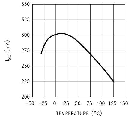
Figure 5-32. Instantaneous Short-Circuit Current versus Temperature (Legacy chip)
