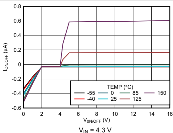
Figure 5-39. ON/ OFF Pin Current versus V_{ON/OFF} (New Chip)
