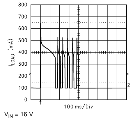
Figure 16. Short-Circuit Current
