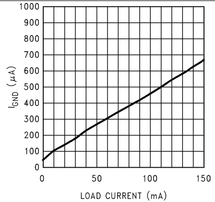
Figure 6. GND Pin vs Load Current
