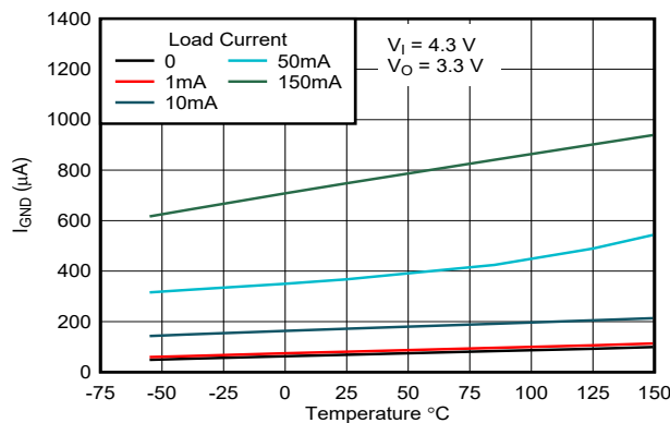
Figure 6-35. Ground-Pin Current vs Temperature for New Chip
