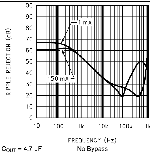
Figure 6. Ripple Rejection
