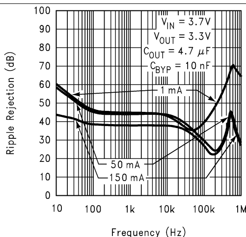
Figure 10. Ripple Rejection
