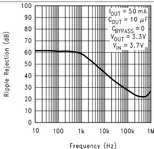
Figure 8. Ripple Rejection
