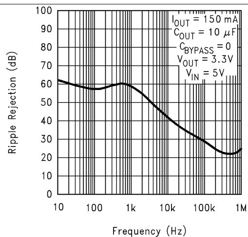
Figure 6. Ripple Rejection
