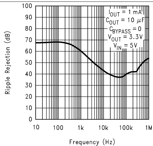
Figure 4. Ripple Rejection
