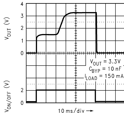
Figure 38. Turnon Time
