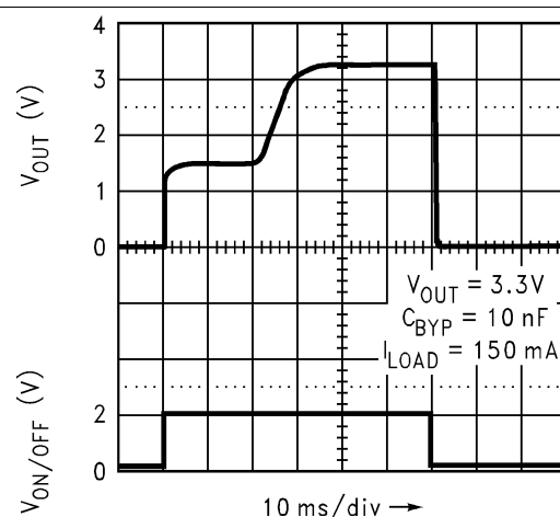
Figure 38. Turnon Time
