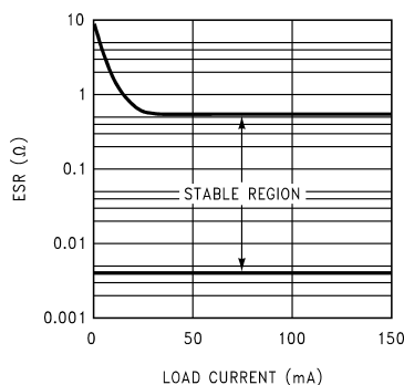
Figure 22. ESR Graph
