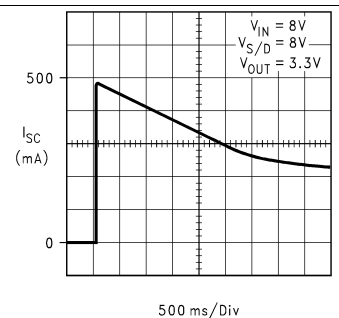
Figure 9. Turnon Waveform
