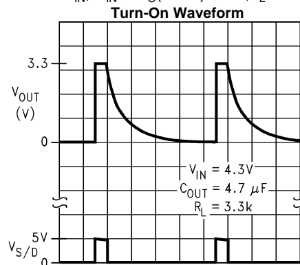
20 \text{ms}/\text{Div} Figure 18.
