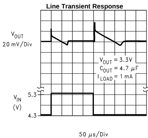
50 \mu\text{s}/\text{Div} Figure 13.
