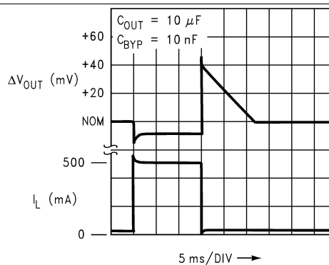
Figure 14. Load Transient Response
