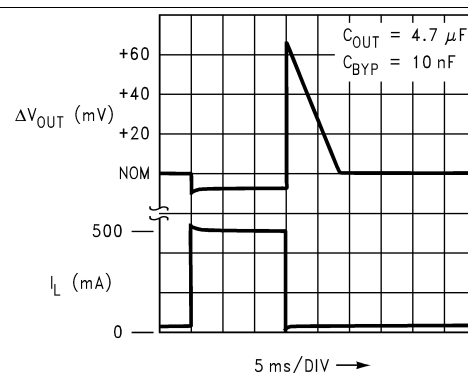
Figure 43. Load Transient Response
