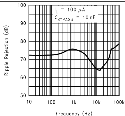
Figure 20. Ripple Rejection
