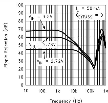
Figure 22. Ripple Rejection
