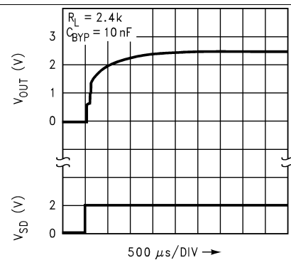
Figure 30. Turn-ON Waveform
