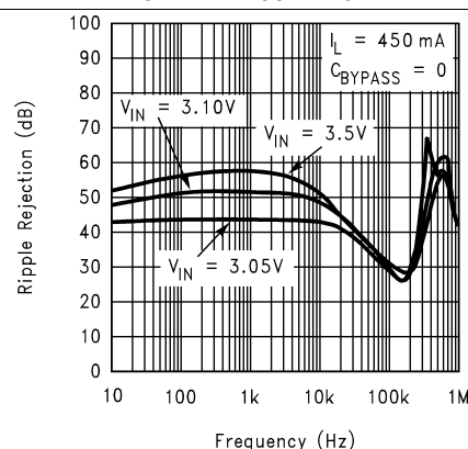
Figure 24. Ripple Rejection
