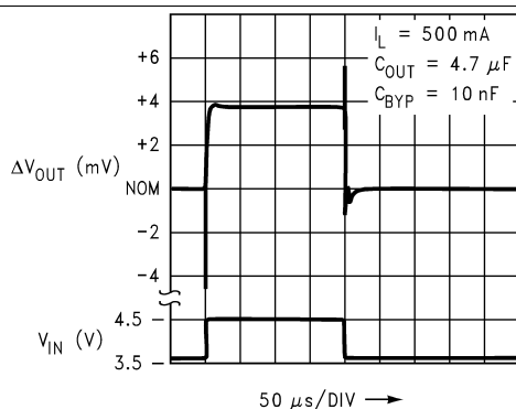
Figure 42. Line Transient Response
