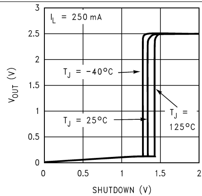
Figure 38. V_{\text{OUT}} vs Shutdown
