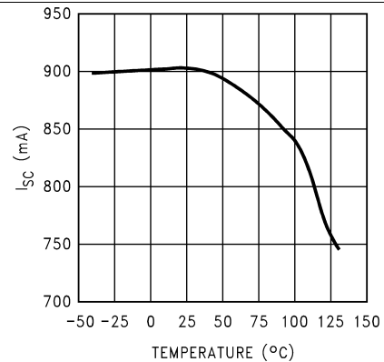
Figure 16. Short Circuit Current vs Temperature
