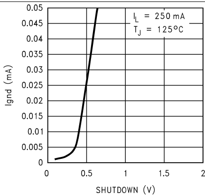
Figure 37. I_{\text{GND}} vs Shutdown
