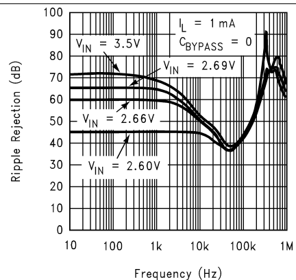
Figure 21. Ripple Rejection
