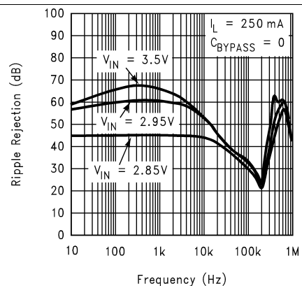
Figure 23. Ripple Rejection
